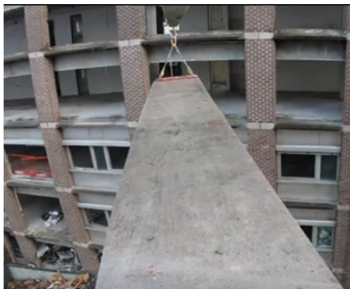
Hoisting the hollow core slabs out of R4. Video clip from NRK
